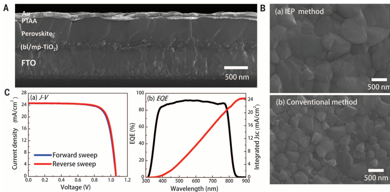
Fig. 2. SEM observations and J - V and EQE measurements. (A) Cross-sectional FESEM image of the device consisting of FTO-glass/ \text{bi-TiO}_2 / \text{mp-TiO}_2 /perovskite/PTAA/Au. (B) The comparison of FESEM surface images of \text{FAPbI}_3 -based layer formed on \text{mp-TiO}_2 by IEP and conventional method. (C) (a) J - V curves of best device measured with a 40-ms scanning delay in reverse (from 1.2 V to 0 V) and forward (from 0 V to 1.2 V) modes under standard AM 1.5G illumination, and (b) EQE spectra for best device and integrated J_{\text{SC}} .
