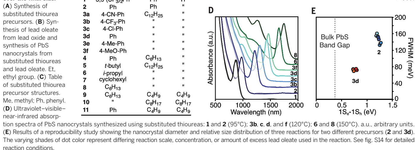
Fig. 2. A library of thioureas can be accessed in a single step and used to prepare PbS nanocrystals with highly reproducible control over the final size.
