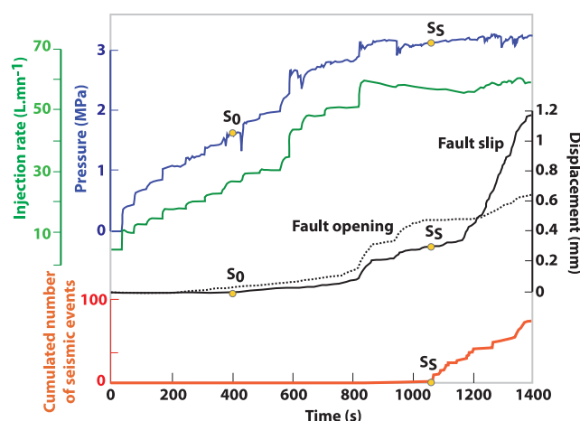
Fig. 2. Fault movements and seismicity induced over time by fluid injection.
