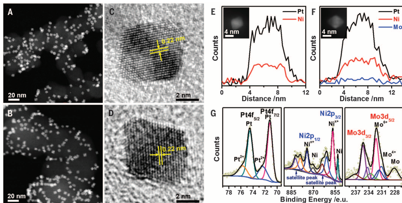
Fig. 1. Schematic illustration of the fabrication process and the structure analyses for the transition metal-doped \text{Pt}_3\text{Ni}/\text{C} catalysts. (A and B) Representative HAADF-STEM images of the (A) \text{Pt}_3\text{Ni}/\text{C} and (B) \text{Mo-Pt}_3\text{Ni}/\text{C} catalysts. (C and D) HRTEM images on individual octahedral (C) \text{Pt}_3\text{Ni}/\text{C} and (D) \text{Mo-Pt}_3\text{Ni}/\text{C} nanocrystals. (E and F) EDS line-scanning profile across individual (E) \text{Pt}_3\text{Ni}/\text{C} and (F) \text{Mo-Pt}_3\text{Ni}/\text{C} octahedral nanocrystals. (G) Pt, Ni, and Mo XPS spectra for the octahedral \text{Mo-Pt}_3\text{Ni}/\text{C} catalyst.
