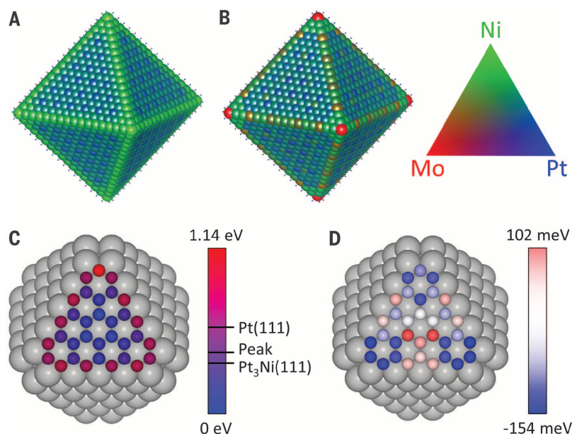
Fig. 4. Computational results. (A and B) The average site occupancies of the second layer of (A) the Ni 117 Pt 3398 NC and (B) the Mo 73 Ni 1143 Pt 3357 NC at 170°C as determined by means of a Monte Carlo simulation. Occupancies are indicated by the color triangle on the right. Small spheres represent the atoms in the outer layer. (C) The calculated binding energies for a single oxygen atom on all fcc and hcp sites on the (111) facet of the Mo 6 Ni 41 Pt 178 NC, relative to the lowest binding energy. Gray spheres represent Pt, and colored spheres represent oxygen sites. Three binding energies are provided for reference: the calculated binding energy on the fcc site of a pure Pt (111) surface, the binding energy corresponding to the peak of the Sabatier volcano (37), and the binding energy on a Pt 3 Ni(111) surface. (D) The change in binding energies when a Ni 47 Pt 178 NC is transformed to a Mo 6 Ni 41 Pt 178 NC by the substitution of Mo on its energetically favored sites in the second layer below the vertices.
