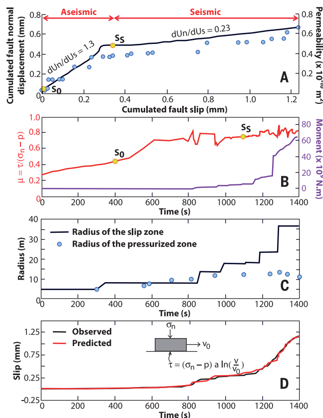
Fig. 3. Estimation of fault permeability and friction law from the in situ hydromechanical data.
