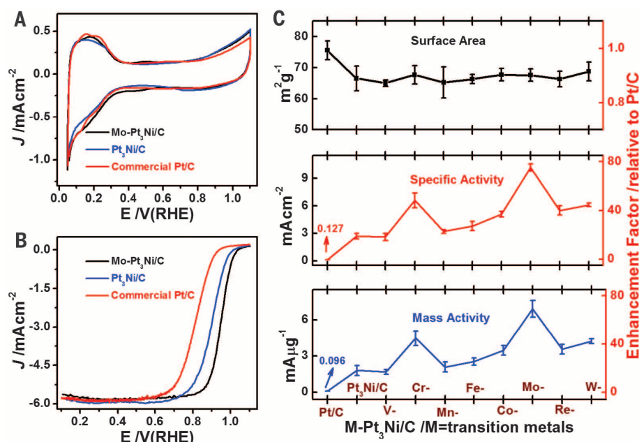
Fig. 2. Electrocatalytic properties of high-performance transition metal-doped octahedral \text{Pt}_3\text{Ni}/\text{C} catalysts and a commercial \text{Pt}/\text{C} catalyst. (A) Cyclic voltammograms of octahedral \text{Mo-Pt}_3\text{Ni}/\text{C} , octahedral \text{Pt}_3\text{Ni}/\text{C} , and commercial \text{Pt}/\text{C} catalysts recorded at room temperature in \text{N}_2 -purged 0.1 M \text{HClO}_4 solution with a sweep rate of 100 mV/s. (B) ORR polarization curves of octahedral \text{Mo-Pt}_3\text{Ni}/\text{C} , octahedral \text{Pt}_3\text{Ni}/\text{C} , and commercial \text{Pt}/\text{C} catalysts recorded at room temperature in an \text{O}_2 -saturated 0.1 M \text{HClO}_4 aqueous solution with a sweep rate of 10 mV/s and a rotation rate of 1600 rotations per min (rpm). (C) The electrochemically active surface area (ECSA, top), specific activity (middle), and mass activity (bottom) at 0.9 V versus RHE for these transition metal-doped \text{Pt}_3\text{Ni}/\text{C} catalysts, which are given as kinetic current densities normalized to the ECSA and the loading amount of Pt, respectively. In (A) and (B), current densities were normalized in reference to the geometric area of the RDE ( 0.196 \text{ cm}^2 ).
