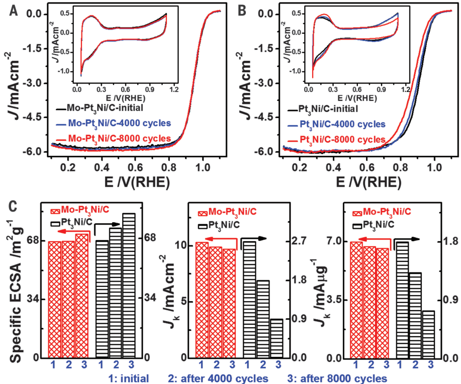
Fig. 3. Electrochemical durability of the high-performance octahedral \text{Mo-Pt}_3\text{Ni}/\text{C} catalyst and octahedral \text{Pt}_3\text{Ni}/\text{C} catalyst. (A and B) ORR polarization curves and (inset) corresponding cyclic voltammograms of (A) the octahedral \text{Mo-Pt}_3\text{Ni}/\text{C} catalyst and (B) the octahedral \text{Pt}_3\text{Ni}/\text{C} catalyst before, after 4000, and after 8000 potential cycles between 0.6 and 1.1 V versus RHE. (C) The changes of ECSAs (left), specific activities (middle), and mass activities (right) of the octahedral \text{Mo-Pt}_3\text{Ni}/\text{C} catalyst and octahedral \text{Pt}_3\text{Ni}/\text{C} catalyst before, after 4000, and after 8000 potential cycles. The durability tests were carried out at room temperature in \text{O}_2 -saturated 0.1 M \text{HClO}_4 at a scan rate of 50 mV/s.
