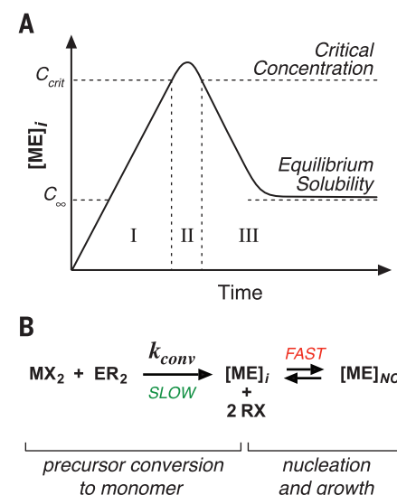
Fig. 1. The mechanism of precursor-limited homogeneous nucleation and growth of colloidal metal chalcogenide nanocrystals. (A) The time evolution of the monomer concentration as described by LaMer and Dinegar, where monomer supersaturation (I) precedes crystal nucleation (II) and is followed by growth (III). (B) Metal and chalcogen precursors ( MX_2 , ER_2 ) react and supply monomers ( [ME]_i ) to the growth medium at a rate that limits the crystallization.
