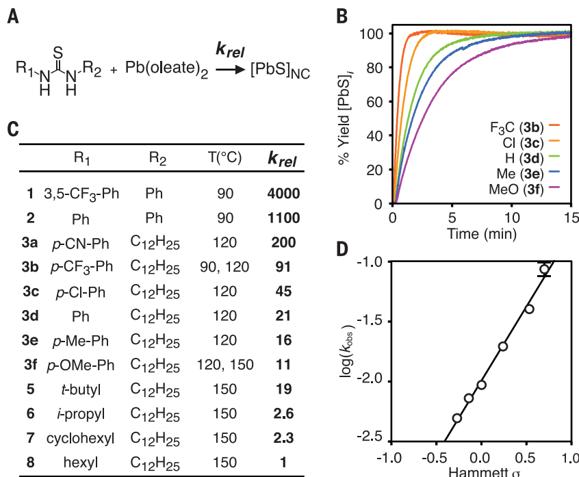
Fig. 3. The reaction of disubstituted thioureas with lead oleate in hexadecane and diphenyl ether follows single exponential kinetics, allowing the conversion rate constants to be quantitatively compared. (A) Schematic of PbS formation reaction used to measure conversion kinetics at 90° to 150°C. (B) Kinetics of lead sulfide formation as measured in situ by the absorbance at \lambda = 400 nm. (C) Effect of thiourea substitution pattern on the relative thiourea conversion rate constants [ k rel ( 1 ) to k rel ( 8 ), e.g., k rel ( 7 ) = k ( 7 )/ k ( 8 )]. The wide range of reactivity requires that kinetics are measured at multiple temperatures. To account for the temperature dependence of the conversion rate constant, 3b and 3f were measured at two temperatures, and the change in rate constant was used to normalize the relative rate constants of the respective temperatures [e.g., k rel ( 3b ) = [ k ( 3b ) 120°C / k ( 8 ) 150°C ] × [ k ( 3f ) 150°C / k ( 3f ) 120°C ]. (D) Hammett plot illustrating the well-defined relationship between the electronic structure of the thiourea and the rate of lead sulfide formation.
