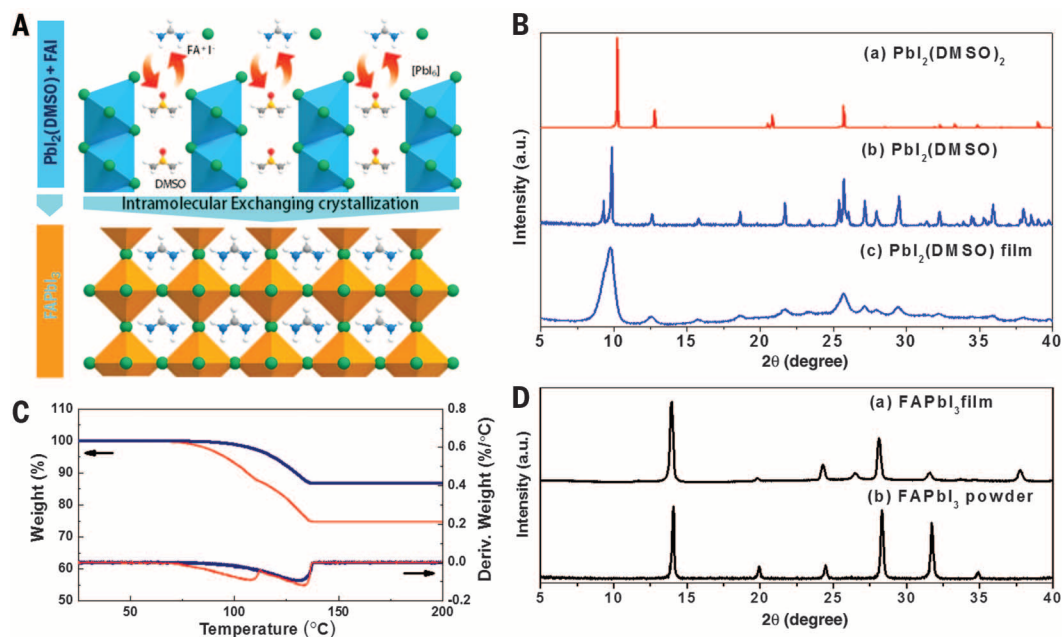
Fig. 1. \text{PbI}_2 complex formation and x-ray diffraction. (A) Schematics of \text{FAPbI}_3 perovskite crystallization involving the direct intramolecular exchange of DMSO molecules intercalated in \text{PbI}_2 with formamidinium iodide (FAI). The DMSO molecules are intercalated between edge-sharing [\text{PbI}_6] octahedral layers. (B) XRD patterns of (a) as-prepared \text{PbI}_2(\text{DMSO})_2 powders, (b) vacuum-annealed \text{PbI}_2(\text{DMSO}) powders, and (c) as-deposited film on fused quartz substrate using \text{PbI}_2(\text{DMSO}) complex solution. (C) TGA of \text{PbI}_2(\text{DMSO})_2 (red line) and \text{PbI}_2(\text{DMSO}) (dark blue line). (D) XRD patterns of (a) as-formed film of \text{FAPbI}_3 by IEP, and (b) \text{FAPbI}_3 powder.
