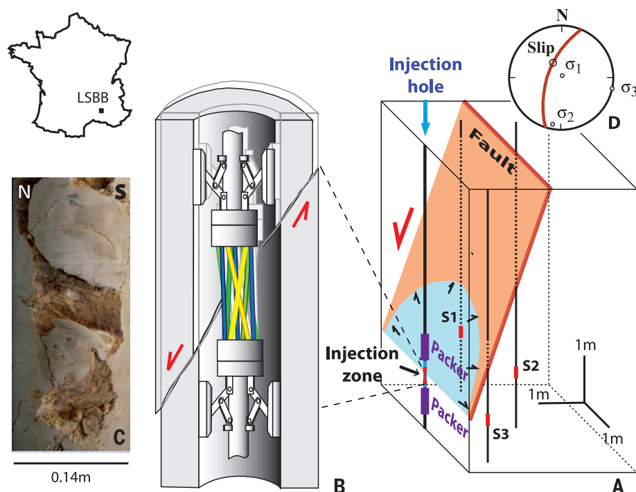
Fig. 1. Experiment setting. (A) Location of the injection interval and the seismometers (S1 to S3) in and around the fault plane. The experiment took place at a depth of 282 m below the Earth's surface, in cretaceous limestone of the southeast France sedimentary basin. (B) Schematic representation of the SIMFIP probe displacement sensor. Deformation of the linkage tubes (colored in yellow, green, and blue) captures the relative displacement of the anchors clamped on the borehole wall in each fault compartment (16). (C) Core from the main slip plane of the fault showing slickensided surfaces, breccia/gouge-rich zones, and a fractured damage zone. (D) Stereographic view of the state of principal stresses, the fault plane, and the fault-parallel slip vector induced by the experiment.
