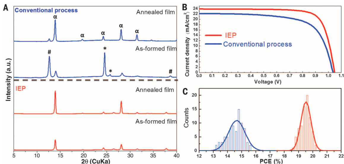
Fig. 3. Comparison of x-ray diffractions, performance, and reproducibility between IEP and conventional process. (A)
