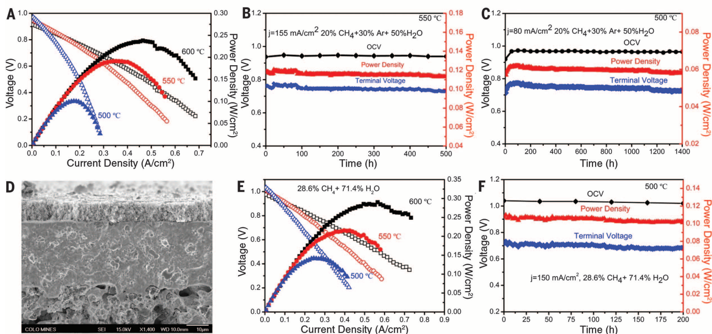
Fig. 4. Performance and microstructure of selected cells under \text{CH}_4/\text{air} operation. (A) I - V and power density for cell 4 under 20 vol. % \text{CH}_4 + 50 vol. % \text{H}_2\text{O} + 30 vol. % \text{Ar}/\text{air} at 500°, 550°, and 600°C; (B) terminal voltage, OCV, and power density at a current density of 155 \text{ mA cm}^{-2} at 550°C for cell 4 under 20 vol. % \text{CH}_4 + 50 vol. % \text{H}_2\text{O} + 30 vol. % \text{Ar}/\text{air} for over 500 hours; (C) terminal voltage, OCV, and power density at a current density of 80 \text{ mW cm}^{-2} at 500°C for
