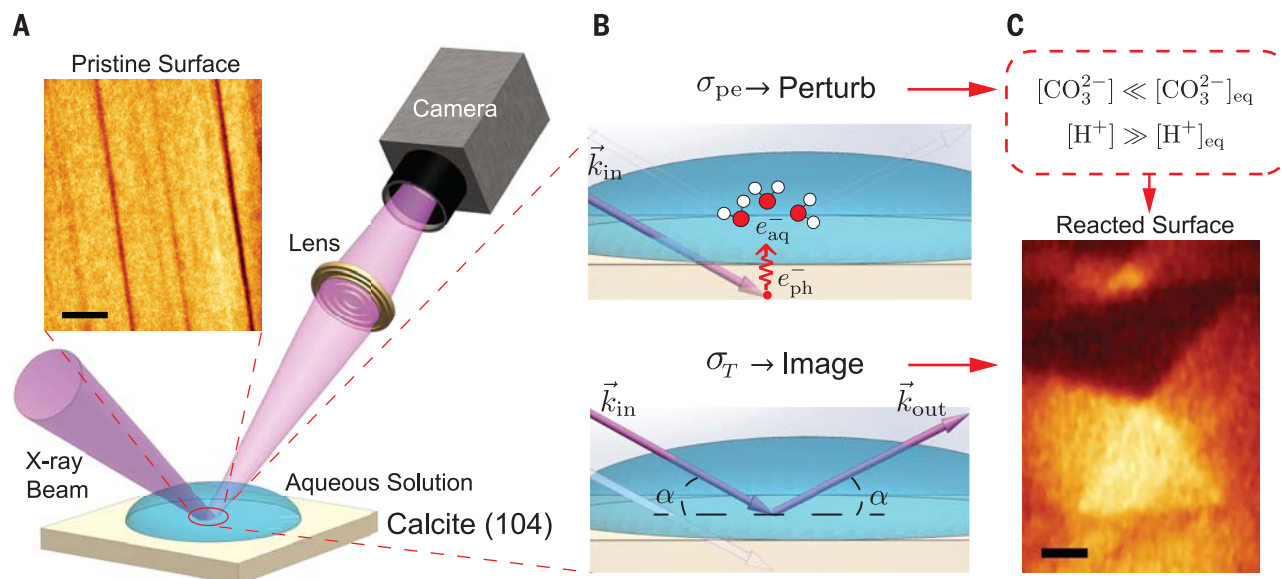
Fig. 1. Imaging the calcite/water interface while simultaneously driving it far from equilibrium. (A) Optical configuration of the x-ray reflection interface microscope. (Inset) XTRM image of steps on a pristine calcite surface. (B) (Top) Photoelectron ( e^-_{ph} ) generated by absorption of an incident x-ray photon in the calcite crystal. The photoelectron propagates to the mineral/water interface and disrupts the local equilibrium through the formation of short-lived radicals and
