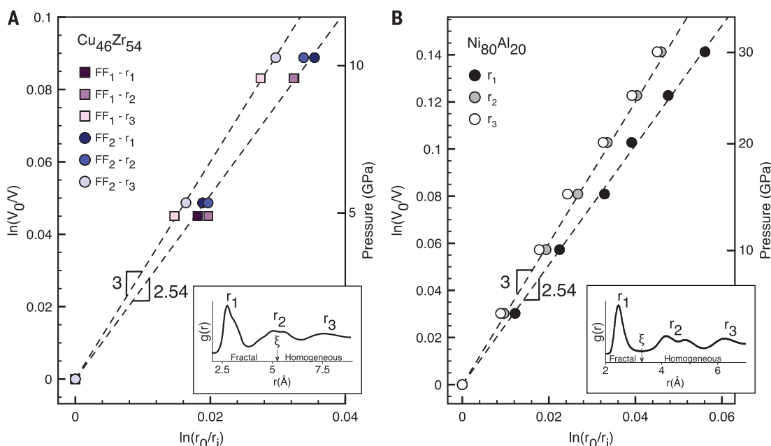
Fig. 2. Dimensionality crossover in simulations. (A) The \text{Cu}_{46}\text{Zr}_{54} from FF1 and FF2 both exhibit a transition in dimensionality from \sim 2.5 to 3 between r_2 and r_3 . (B) \text{Ni}_{80}\text{Al}_{20} exhibits a transition in dimensionality from \sim 2.5 to 3 between r_1 and r_2 . The insets show corresponding RDF curves with the correlation lengths \xi indicated.
