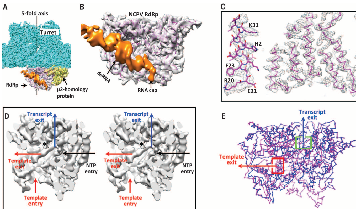
Fig. 2. Structures of the RdRp complexes within NCPV and TCPV. (A) Location of an RdRp within the NCPV capsid (partially shown). The RdRp density map (gray) is superimposed on its \alpha model (magenta). (B) Zoomed-in view of the NCPV RdRp in (A). The \mu 2-homology protein is removed for clarity. (C) Partial view of the density map (mesh) of the RdRp superimposed on its \alpha model. Several N-terminal \alpha helix residues (left) are shown (National Center for Biotechnology Information accession number AF323782). K, Lys; H, His; F, Phe; R, Arg; E, Glu. (D) Cut-open view (cross-eye stereo view) showing the four channels in the TCPV RdRp. Asterisks denote the location of the switch loop. (E) \alpha model of the NCPV RdRp (magenta) superimposed on that of the TCPV RdRp (blue).
