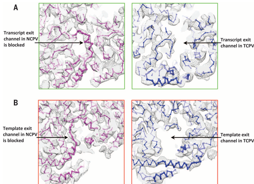
Fig. 3. Conformational changes between RdRps of NCPV and TCPV. \alpha models are shown in bold. (A) Zoomed-in view of the transcript exit channels in the NCPV and TCPV RdRps shown in Fig. 2E. The transcript exit channel in NCPV is blocked by an \alpha helix from the bracelet domain. (B) Zoomed-in view of the template exit channels in NCPV and TCPV RdRps. The template exit channel in NCPV is blocked by two \alpha helices from the bracelet domain.
